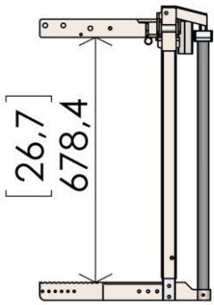
DIMENSION CLOSED FOR (49,9) In 1267 Open
