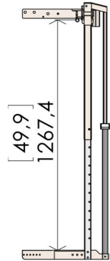
(63,05) In, 1600 mm ON REQUEST
